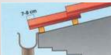
Fig. 3 The first row of tiles must overhang the guttering for about one third of the width of the gutter itself.
